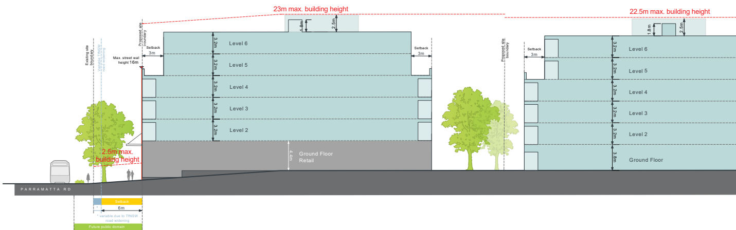
Figure K20-28 Built Form Envelope - Section I
