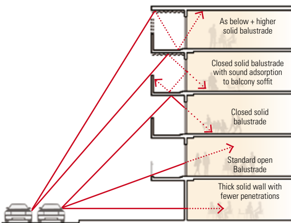
Figure K20-39 Noise mitigating facade treatments (Source: Development Near Rail Corridors And Busy Roads Interim Guideline, NSW)
