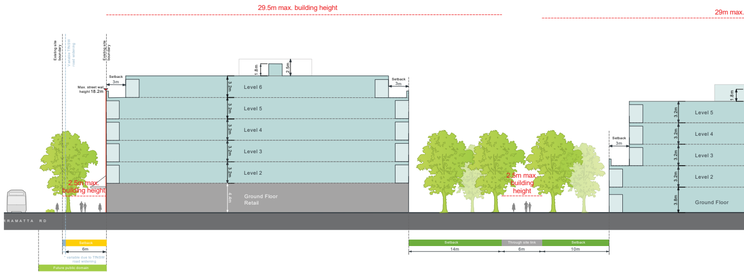
Figure K20-27 Built Form Envelope - Section H
